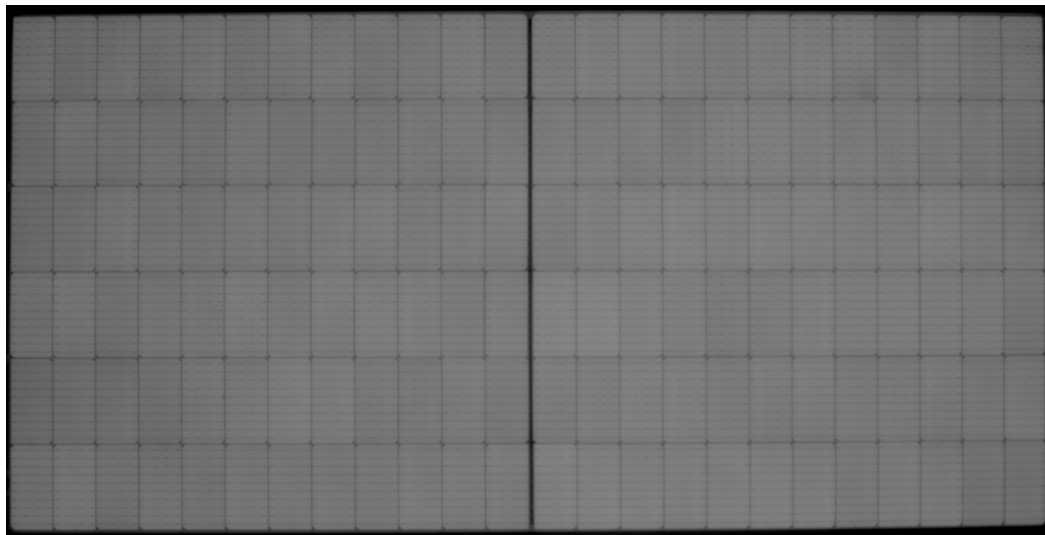
Fig. 6 EL photo of module No.2 Serial number: AS22200108899
